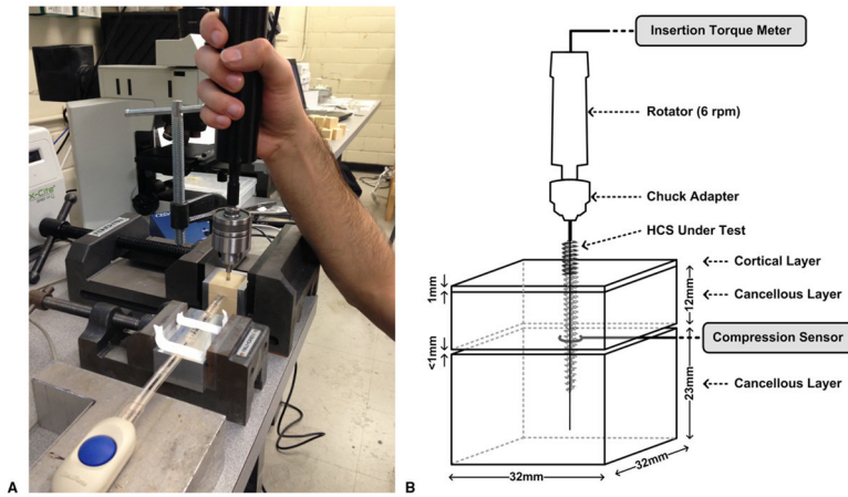
FIGURE 2. Test setup. A Photograph. B Schematic.
