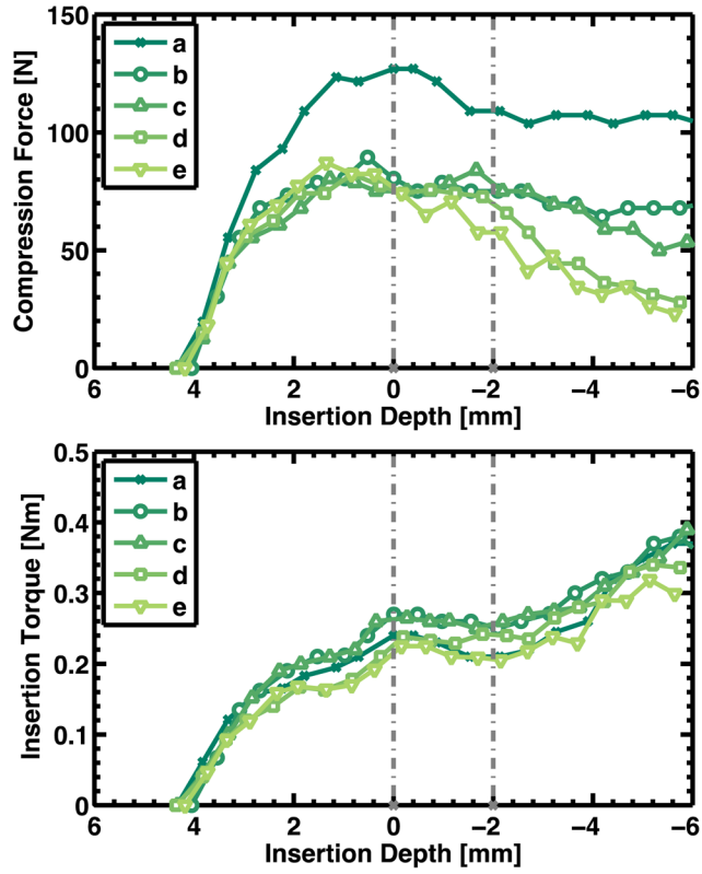
FIGURE 3. Individual tests (a– e) of the Herbert-Whipple screw: interfragmentary compression profile (top) and insertion torque profile (bottom). Markers represent measurement points taken between half-turns of the screw. Insertion depth is the distance between the proximal tip of the screw and the surface of the bone (foam). Vertical hashed lines represent the screw position when the proximal tip is flush (0 mm) and buried (–2 mm) below the cortex.
